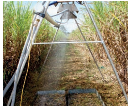
Rainfall simulator in cane paddock
